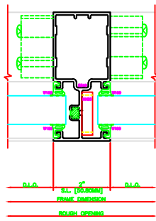
648 EXPANSION VERTICAL S433 SHEARLOCK
